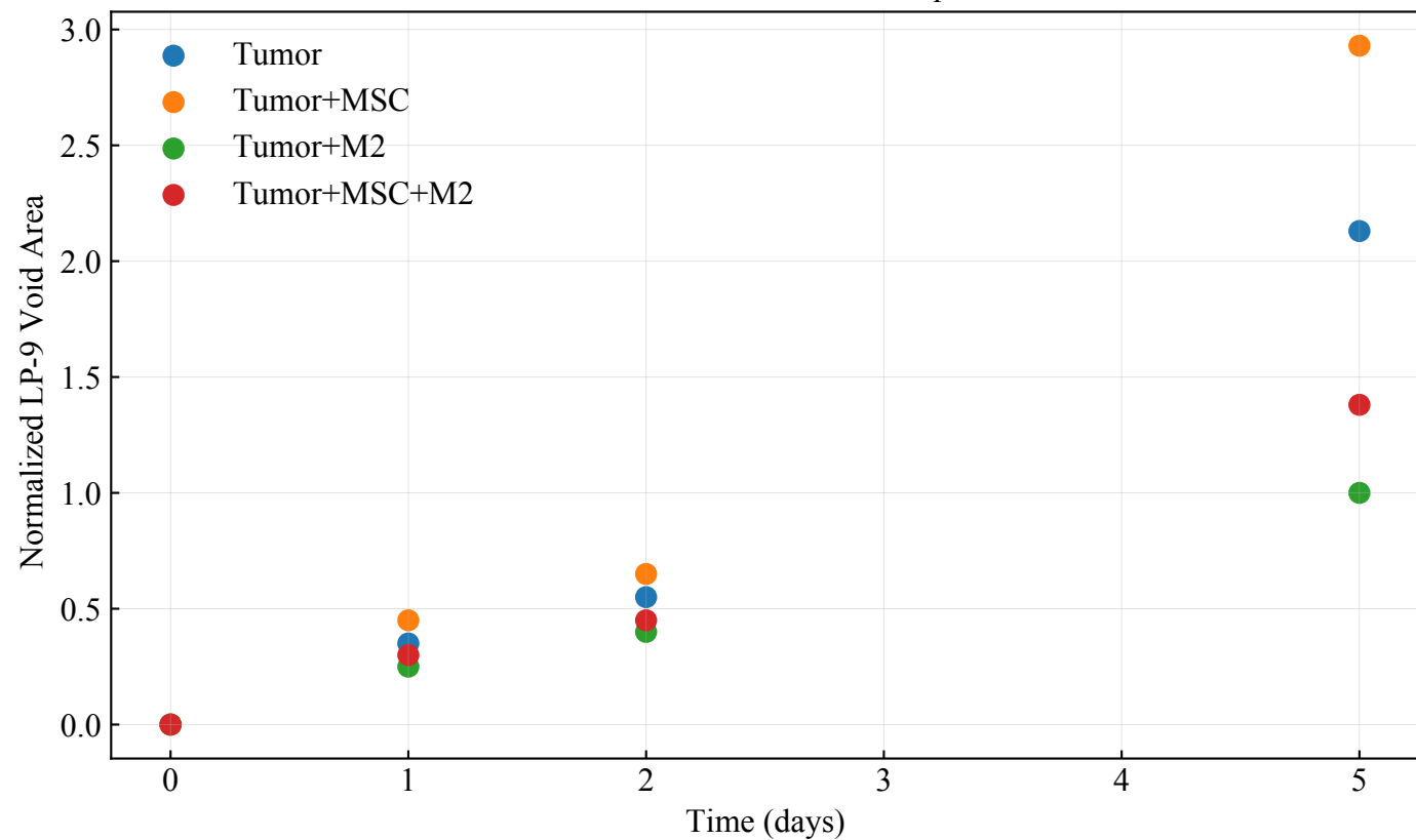
LP-9 Void Normalized to OVCAR4 Spheroid Area
